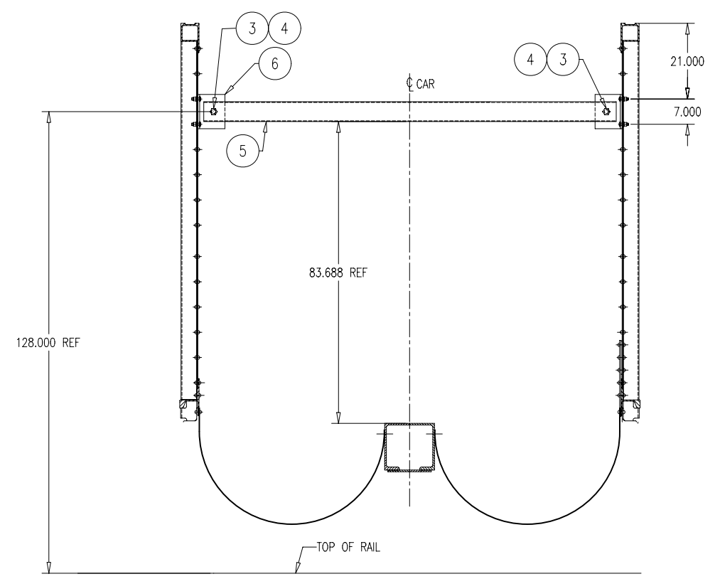
SECTION "A"-"A" TYPICAL AT STAKES #3, #7, AND #11
