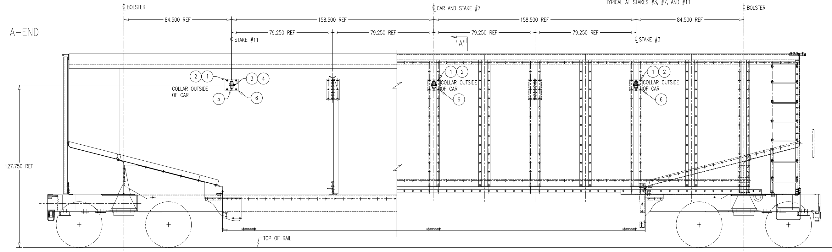
SECTION "A"-"A" TYPICAL AT STAKES #3, #7, AND #11
